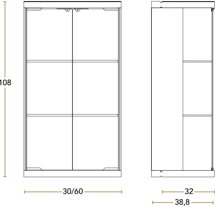
Vetrina Verticale Vertical Display Cabinet
