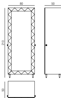
4005 Mobile ingresso Entrance cabinet
