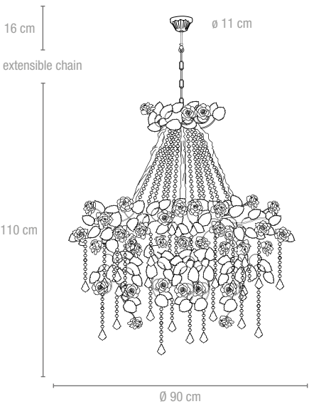
Lady Chatterley Chandelier code 4024559 30 kg type 12 lights electrification 12 x Max 28W E14 CE
