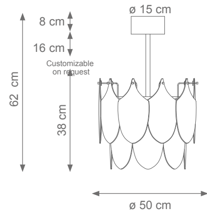
Tiny Short Peacock Chandelier (2 levels, 18 feathers) Code: F807911 Type 6 lights electrification x Max 28W E14 CE Size: cm. 38 h x 50 ø - 18 kg
