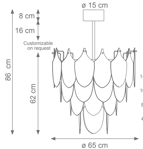
Mini Peacock Chandelier (4 levels, 36 feathers ) Code: F807912 Type 9 lights electrification x Max 28W E14 CE Size: cm. 62 h x 65 ø - 35 kg
