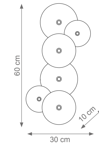
Medium Dandelion Wall Light Code: F807768 Type 3 lights electrification x Max 28W G9 CE Size: cm. 60 h x 30 l x 10 w - 5 kg
