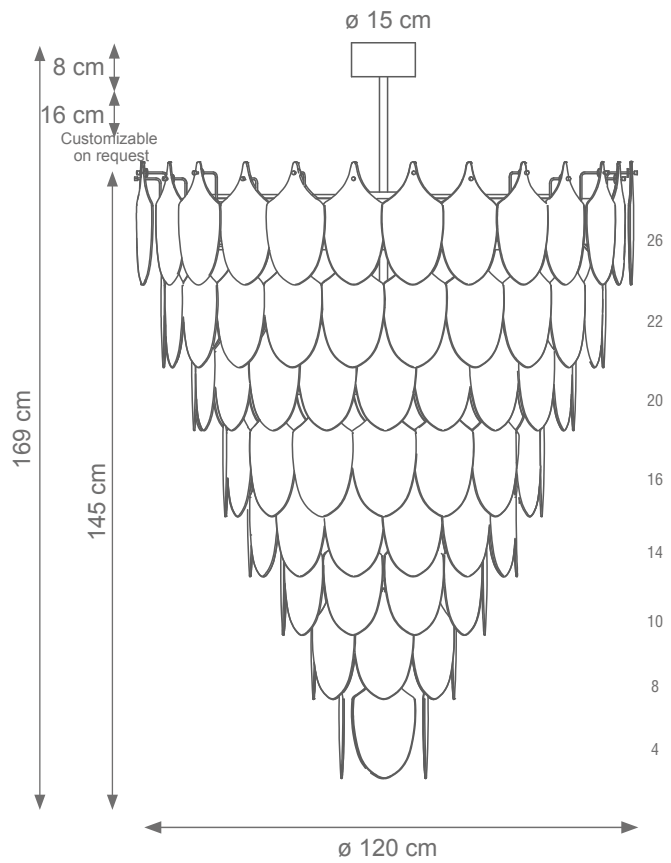
Big Peacock Chandelier (8 levels, 120 feathers) Code F807553 Type 18 lights electrification x Max 28W E14 CE Size: cm. 145 h x 120 ø - 105 kg
