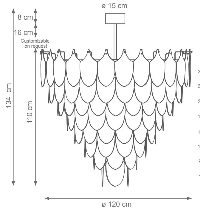
Large Peacock Chandelier (8 levels, 120 feathers) Code F807276 Type 18 lights electrification x Max 28W E14 CE Size: cm. 110 h x 120 ø - 105 kg
