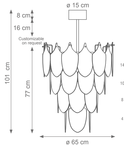
Mignon Peacock Chandelier (4 levels, 36 feathers) Code: F807651 Type 9 lights electrification x Max 28W E14 CE Size: cm. 77 h x 65 ø - 35 kg
