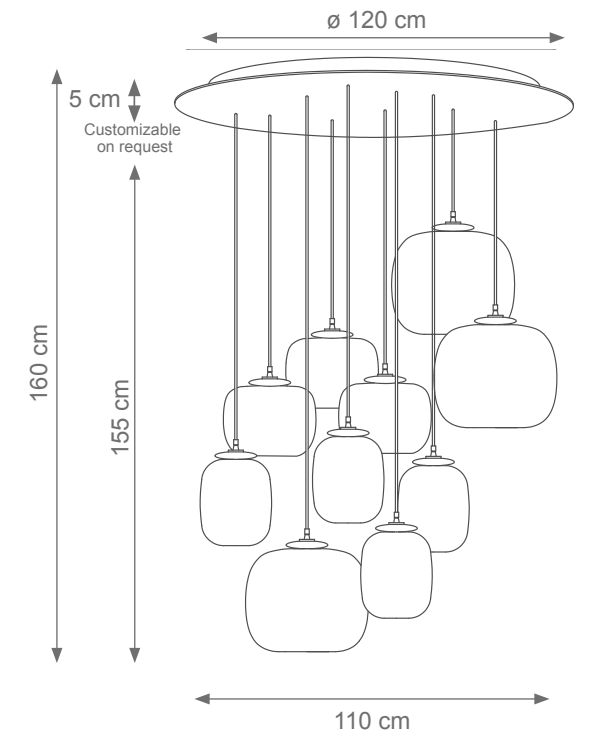
Grand Salento Chandelier Code: F808195 Type 10 lights electrification x Max 28W E14 CE Size: cm. 160 h x 120 \varnothing - 72 kg
