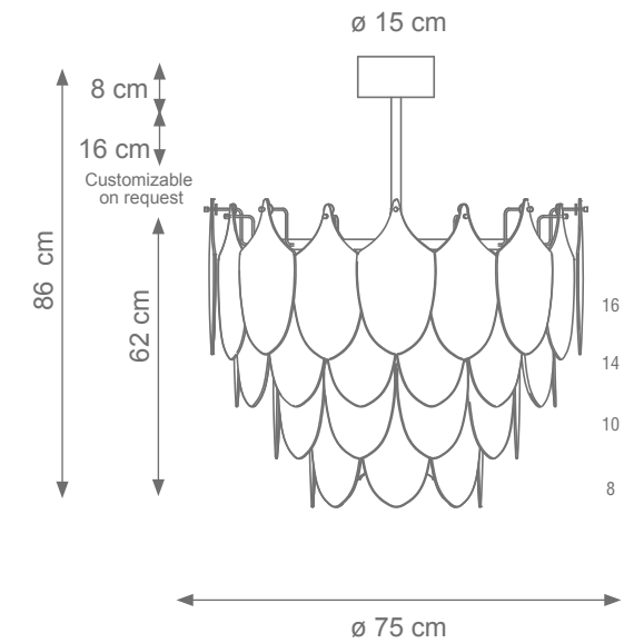
Small Short Peacock Chandelier (4 levels, 48 feathers) Code: F807561 Type 9 lights electrification x Max 28W E14 CE Size: cm. 62 h x 75 ø - 45 kg
