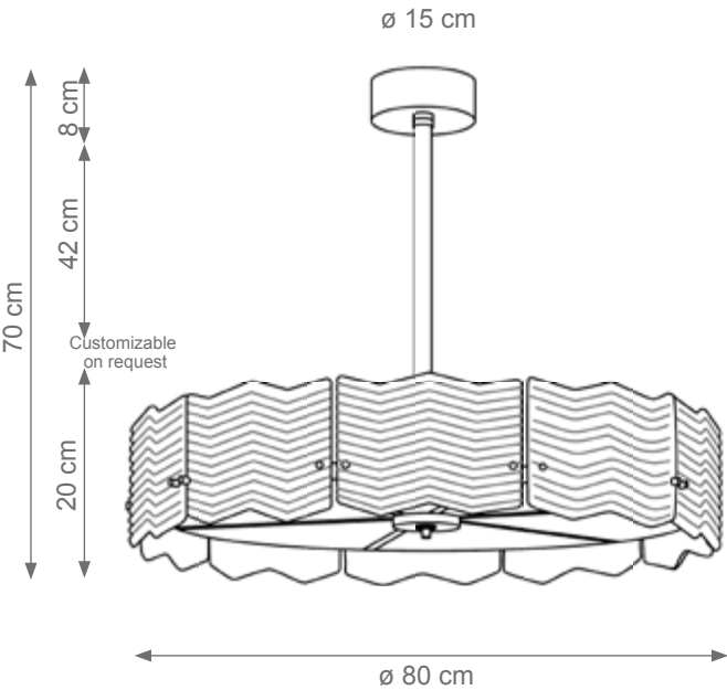
Kate Chandelier Code: F807904 Type 6 lights electrification x Max 28W E14 CE Size: cm. 20 h x 80 ø - 32 kg
