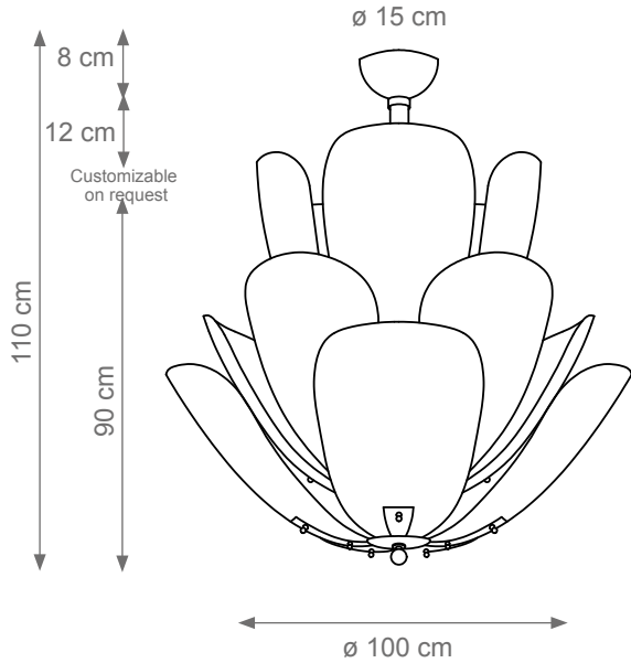
Victoria Chandelier Code: F808419 Type 15 lights electrification x Max 28W LED G9 CE Size: cm. 90 h x 100 ø - 50 kg
