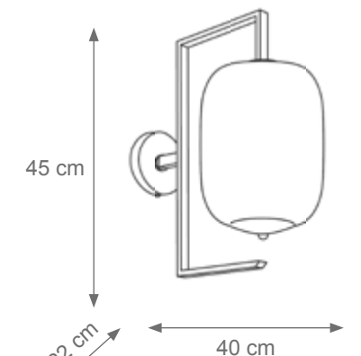
Soho Wall Light Code: F808272 Type 1 light electrification x Max 28W E14 CE Size: cm. 45 h x 40 l x 22 w - 4 kg
