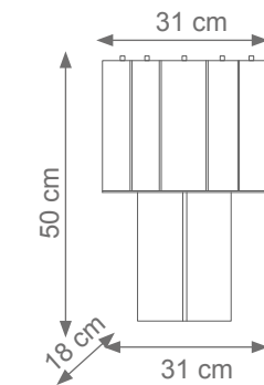
Drum Wall Light Code: F807332 Type 2 lights electrification x Max 28W E14 CE Size: cm. 50 h x 31 l x 18 w - 4,5 kg
