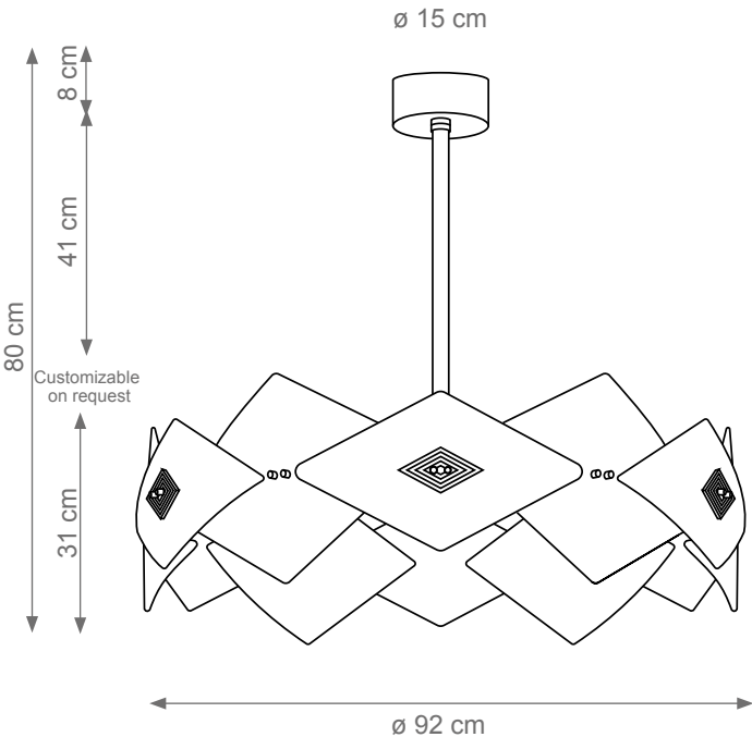
Rombo Chandelier Code: F807702 Type 6 lights electrification x Max 28W E14 CE Size: cm. 31 h x 92 ø - 36 kg
