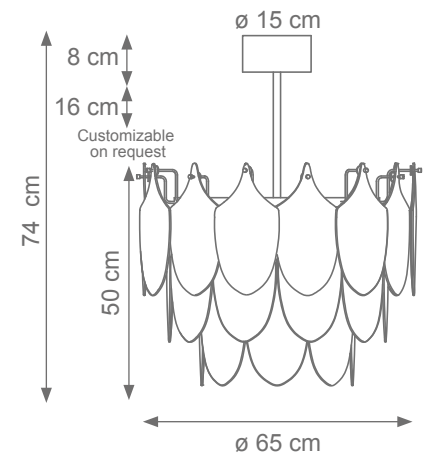
Mini Short Peacock Chandelier (3 levels, 32 feathers) Code: F807821 Type 9 lights electrification x Max 28W E14 CE Size: cm. 50 h x 65 ø - 30 kg
