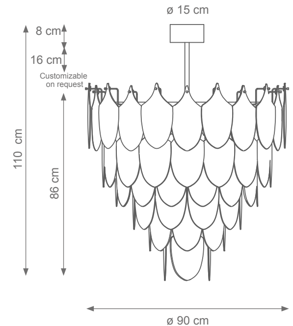
Medium Peacock Chandelier (6 levels, 72 feathers) Code: F807277 Type 12 lights electrification x Max 28W E14 CE Size: cm. 86 h x 90 ø - Max 70 kg
