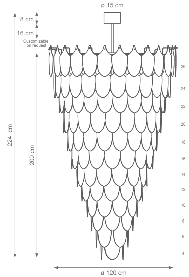
King Peacock Chandelier (12 levels, 180 feathers) Code F807558 Type 24 lights electrification x Max 28W E14 CE Size: cm. 200 h x 120 ø - 155 kg
