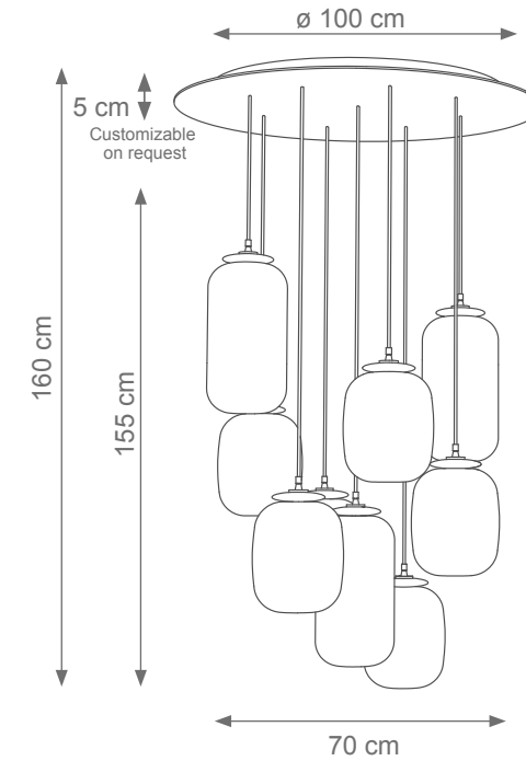
Long Island Chandelier Code: F807827 Type 9 lights electrification x Max 28W E14 CE Size: cm. 160 h x 100 \varnothing - 60 kg
