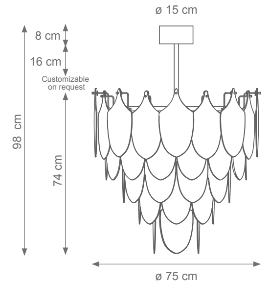
Small Peacock Chandelier (5 levels, 52 feathers) Code: F807819 Type 9 lights electrification x Max 28W E14 CE Size: cm. 74 h x 75 ø - 50 kg
