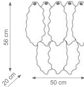
Large Kelly Wall Light Code F808583 Type 4 lights electrification x Max 28W E14 CE Size: cm. 56 h x 50 l x 20 w - 8 kg
