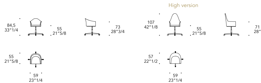
PEGGY OFFICE ALTA Base regolabile in altezza con ruote. Base with pump to adjust the height and with wheels.
