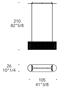
Suspended Lamp Oval
